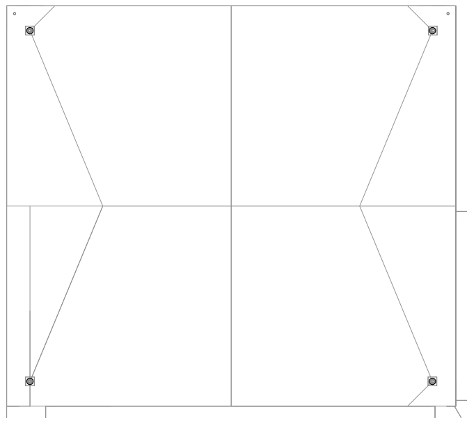
① GYM ROOF 1/8" = 1'-0"
