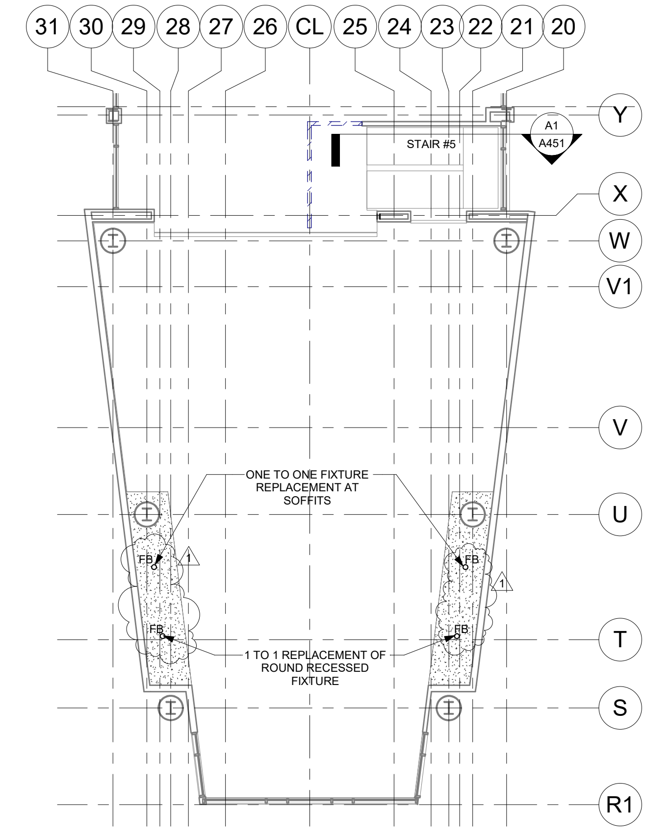
A1 SECOND FLOOR REFLECTED CEILING PLAN 1/8" = 1'-0"
