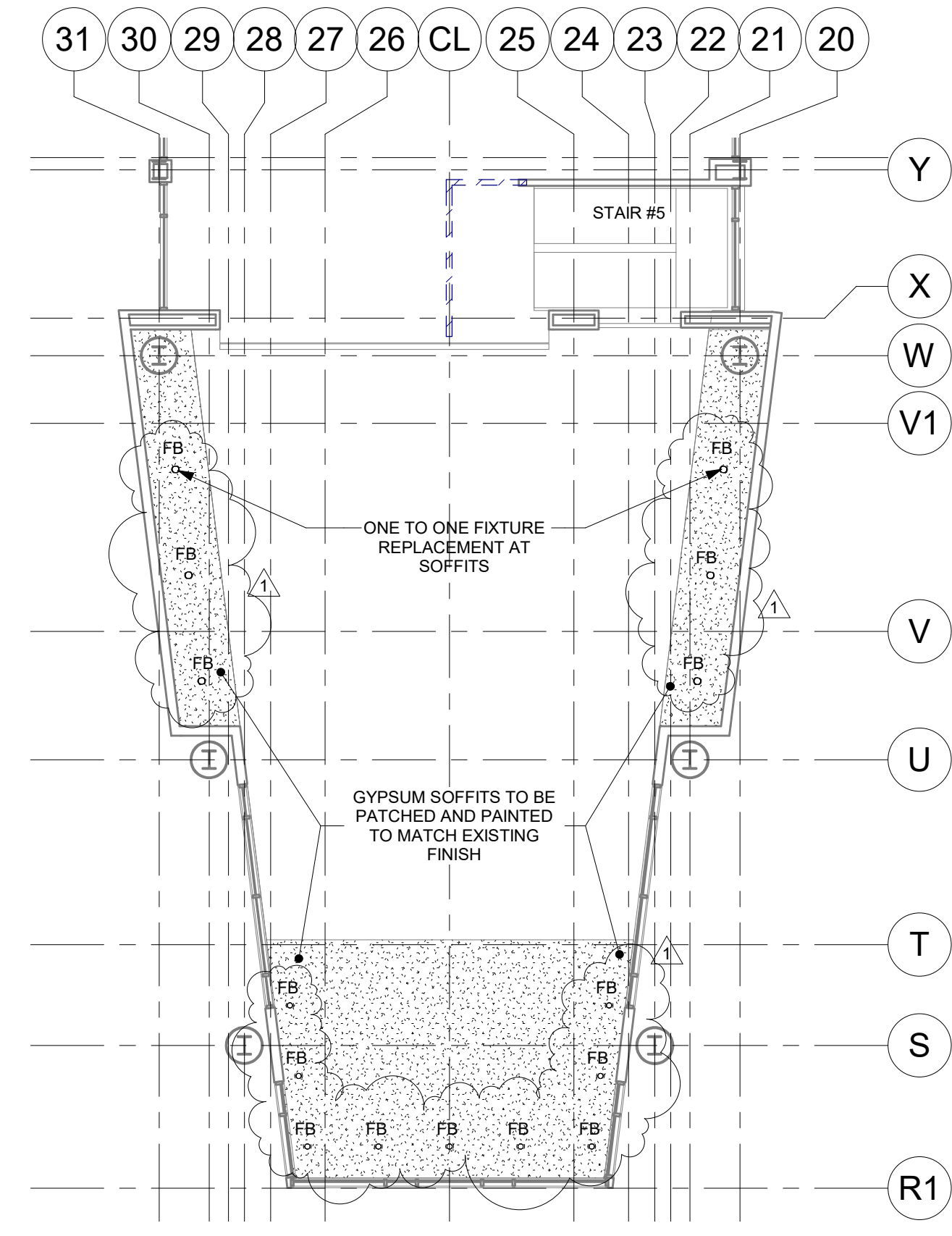
A4 THIRD FLOOR REFLECTED CEILING PLAN 1/8" = 1'-0"
