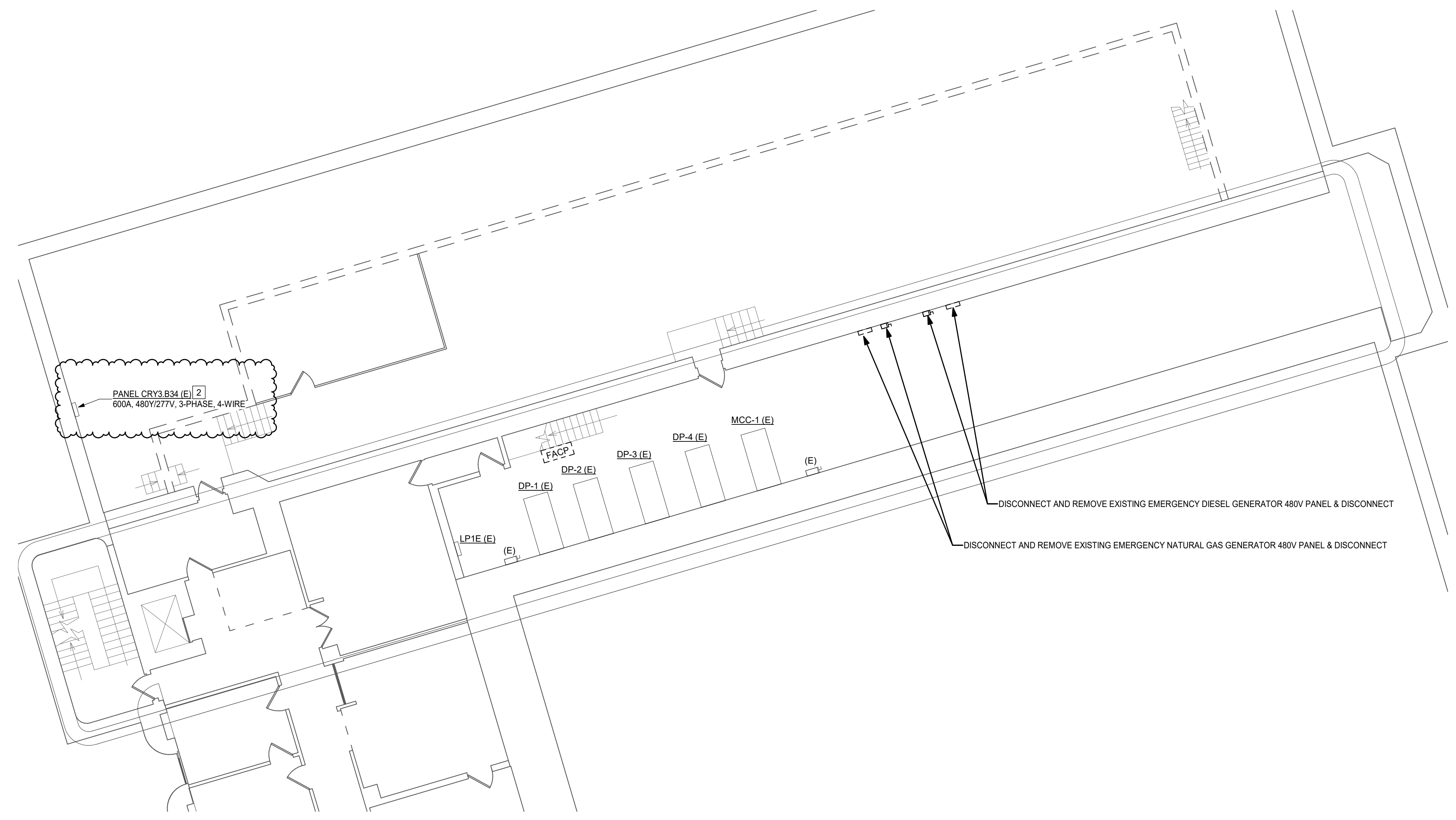
1 Partial Third Floor Demolition Plan - ELEC 1/8" = 1'-0"
